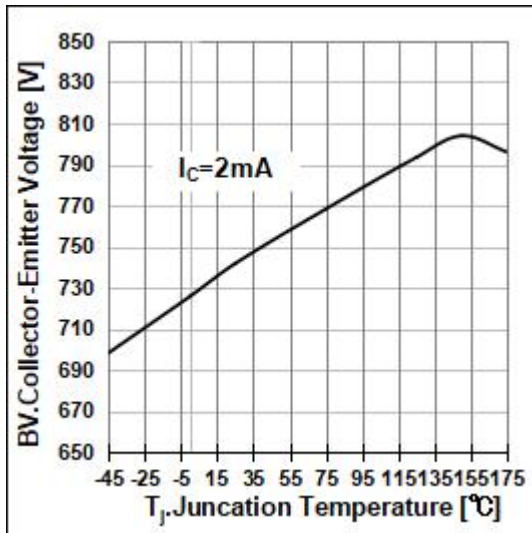
Fig1. Collector-Emitter Breakdown Voltage Temperature characteristic
