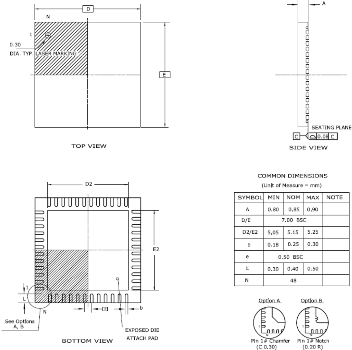
Figure 10-8. QFN-48 Package Drawing for ATSAM4LC4/2 and ATSAM4LS4/2
