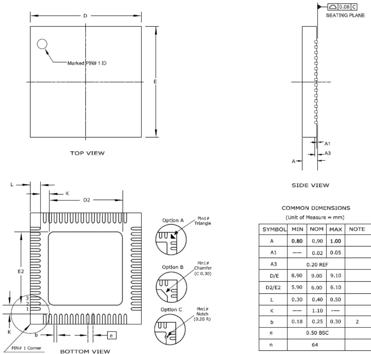
Figure 10-6. QFN-64 Package Drawing
