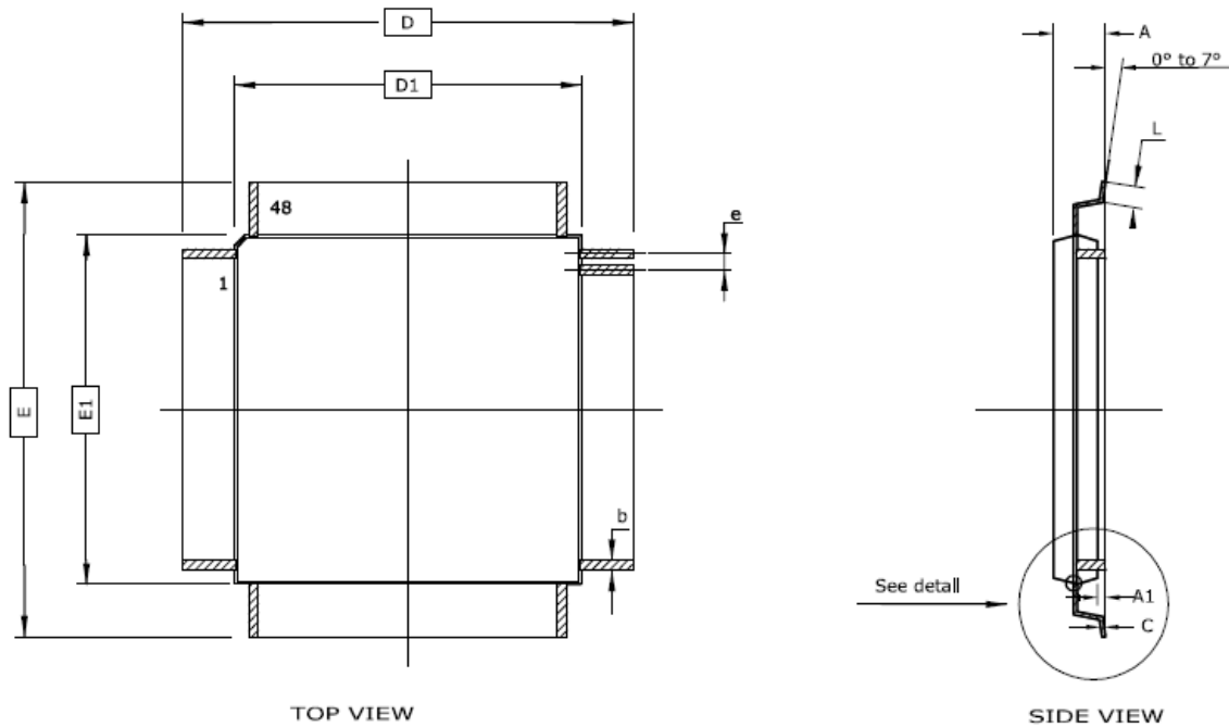
Figure 10-7. TQFP-48 (ATSAM4LC4/2 and ATSAM4LS4/2 Only) Package Drawing
