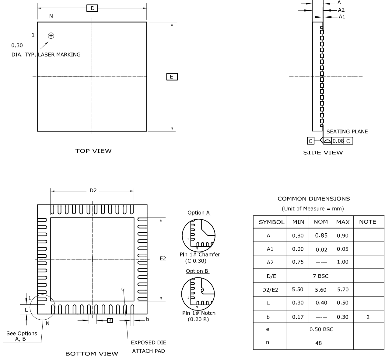
Figure 10-9. QFN-48 Package Drawing for ATSAM4LC8 and ATSAM4LS8
