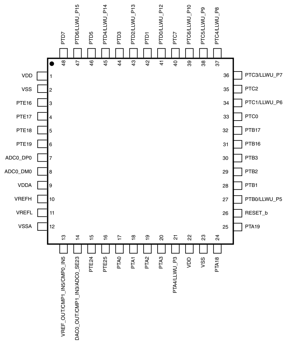
Figure 24. K02F 48 LQFP pinout diagram
