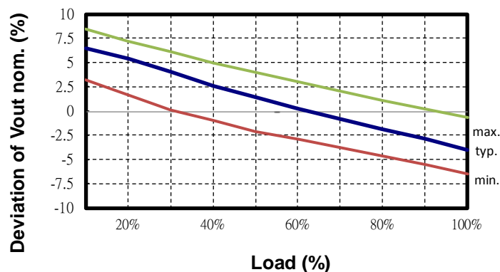
5VDC Output
