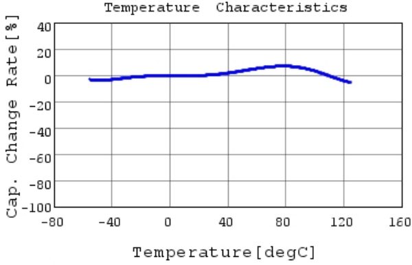
GRM155R70J105MA12 C-Temp. capchange, DC0.0V,
