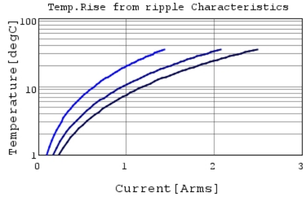
GRM188R7YA474KE05 Temp.rise — 200kHz
