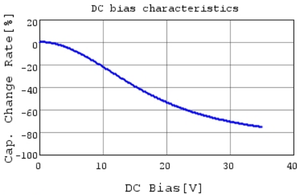
GRM188R7YA474KE05 C-DC bias capchange, 25.0c
