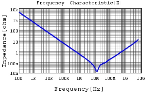
GRM188R7YA474KE05 |Z| DCOV, 25degC
