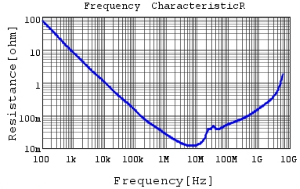
GRM188R7YA474KE05 R DCOV, 25degC
