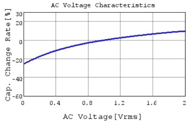
GRM188R7YA474KE05 C-AC Voltage capchange, Dc
