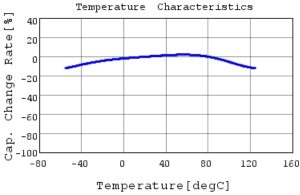
GRM188R7YA474KE05 C-Temp. capchange, DC0.0V,
