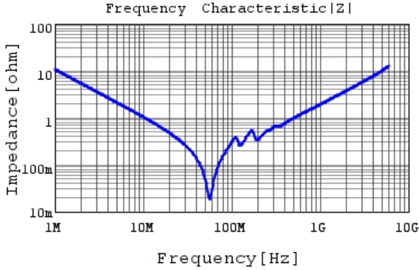
GRM2195C1H153JA01 |Z| DCOV, 25degC
