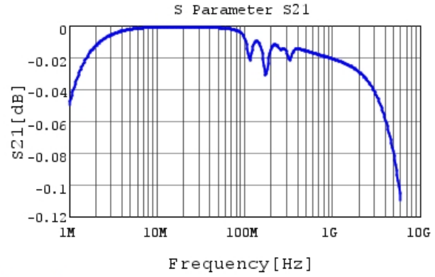
GRM2195C1H153JA01 S21 DCOV, 25degC
