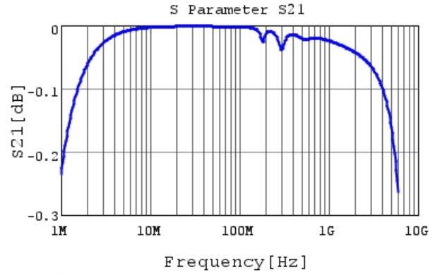
GRM2195C1H682JA01 S21 DCOV, 25degC
