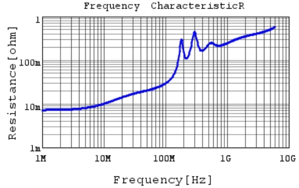
GRM2195C1H682JA01 R DCOV, 25degC
