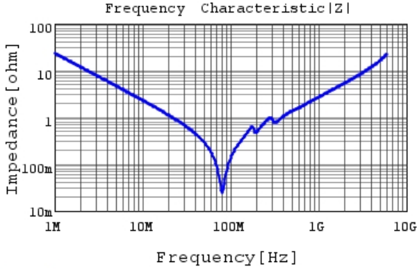
GRM2195C1H682JA01 |Z| DCOV, 25degC
