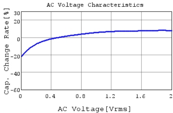
GRM21BZ71A226ME15 C-AC Voltage capchange, Dc
