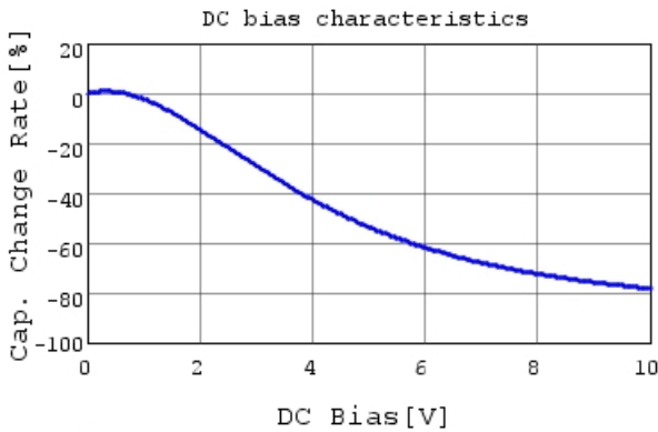
GRM21BZ71A226ME15 C-DC bias capchange, 25.0c
