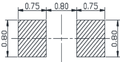
推荐焊盘尺寸 Recommended Soldering Pad
