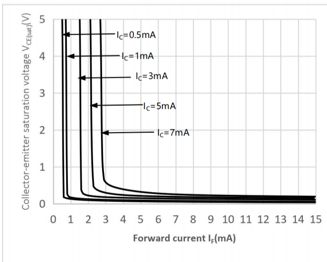
Fig.11 Collector-emitter Saturation Voltage vs Forward Current
