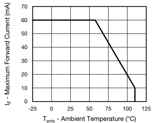
Fig. 2 - Maximum Forward Current vs. Ambient Temperature
