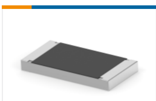
TE Part #1-2176350-6 CRGCQ 2512 330R 5%
