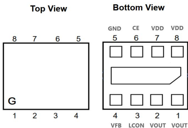
DFN1216-8 Pin Configuration
