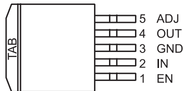
Fig. 2. 5-Pin TO-263 (D 2 Pak) Adjustable Voltage
