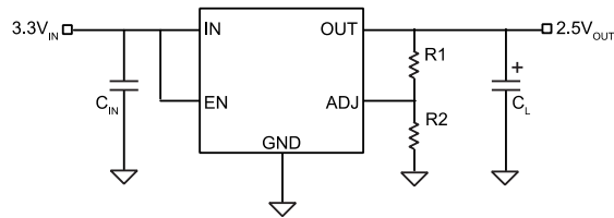
Fig. 1. MIC29302 Adjustable Output Regulator
