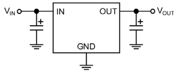
Fig. 3. Linear Regulators Require Only Two Capacitors for Operation
