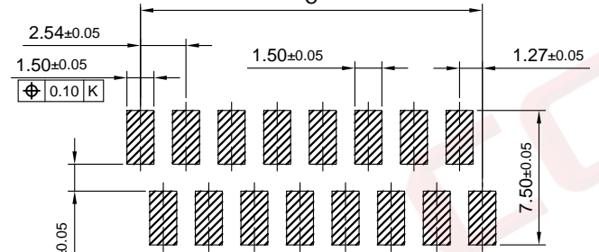
Recommended PC-Board layout (Component side of board shown)
