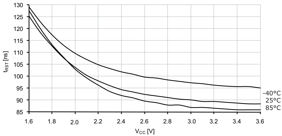
Figure 37-232. Minimum Reset pin pulse width vs. V CC .
