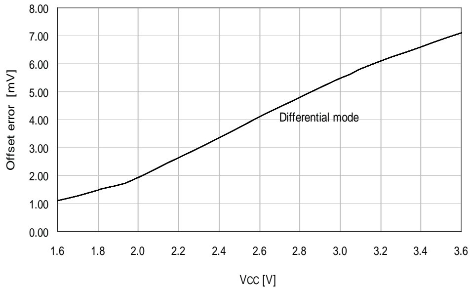
Figure 33-325. Offset error vs. V_{CC} .
