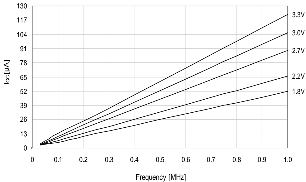
Figure 33-159. Idle mode supply current vs. frequency. f_{SYS} = 0 - 1MHz external clock, T = 25°C .
