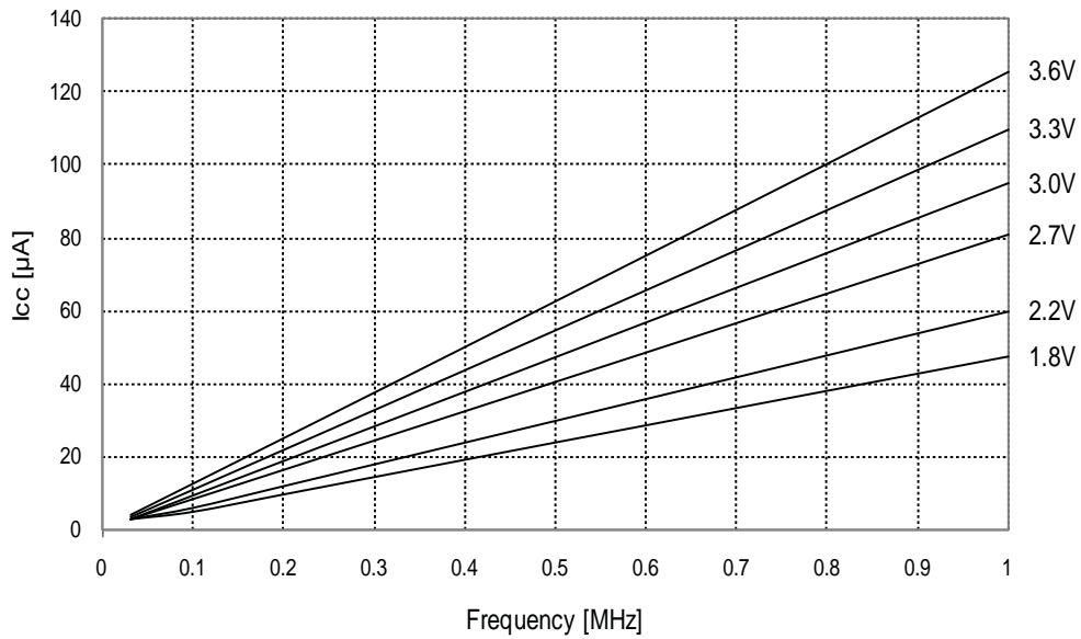
Figure 33-92. Idle supply current vs. frequency. f_{SYS} = 0 - 1.0MHz , T = 25^\circ C .
