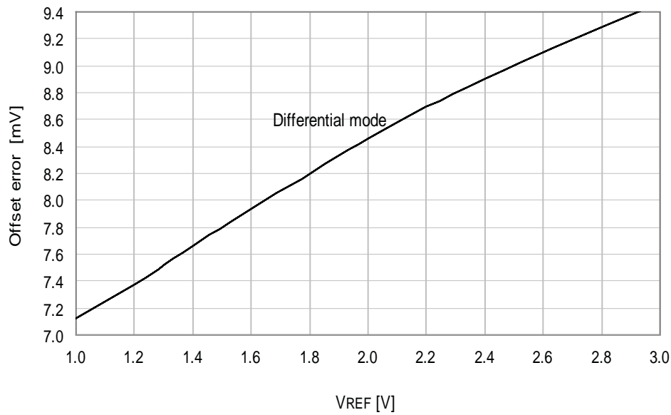
Figure 33-323. Offset error vs. V_{REF} . T = 25^{\circ}\text{C} , V_{CC} = 3.6\text{V} , ADC sample rate = 300kps.
