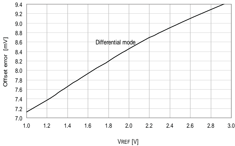
Figure 33-256. Offset error vs. V_{REF} . T = 25^{\circ}\text{C} , V_{CC} = 3.6\text{V} , ADC sample rate = 300ksps.
