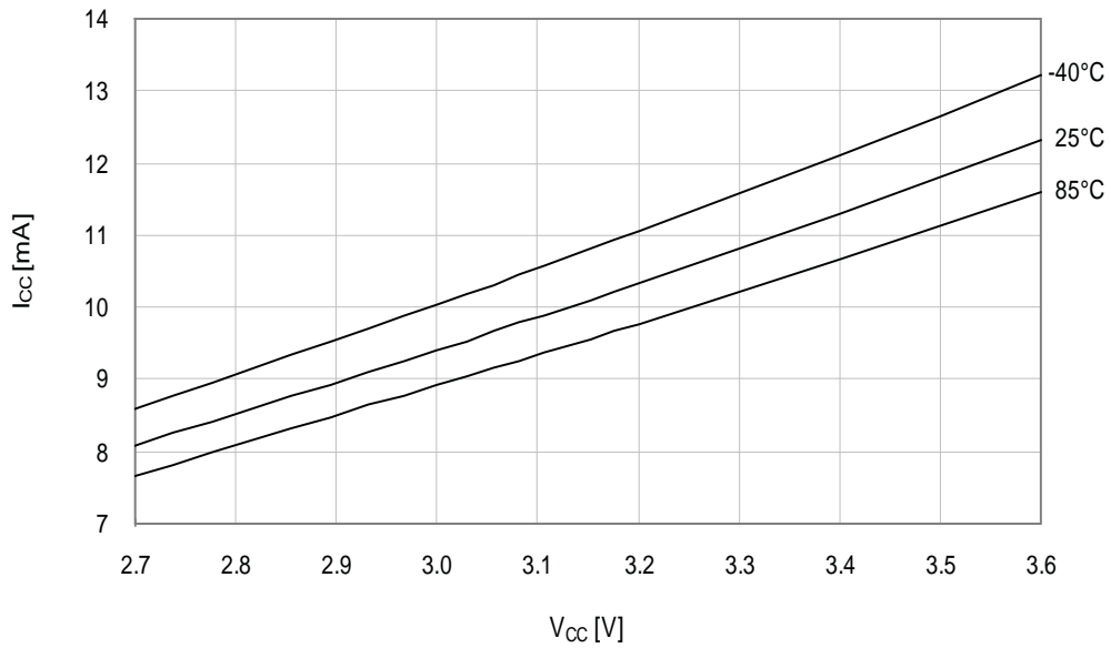
Figure 33-158. Active mode supply current vs. V_{CC} . f_{SYS} = 32MHz internal oscillator.
