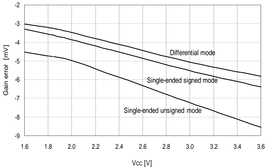
Figure 33-322. Gain error vs. V_{CC} . T = 25^{\circ}\text{C} , V_{REF} = \text{external } 1.0\text{V} , ADC sample rate = 300kps.
