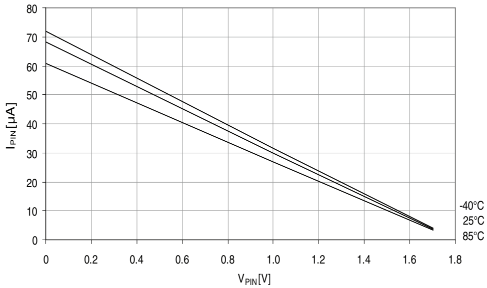
Figure 37-228. Reset pin pull-up resistor current vs. reset pin voltage.
