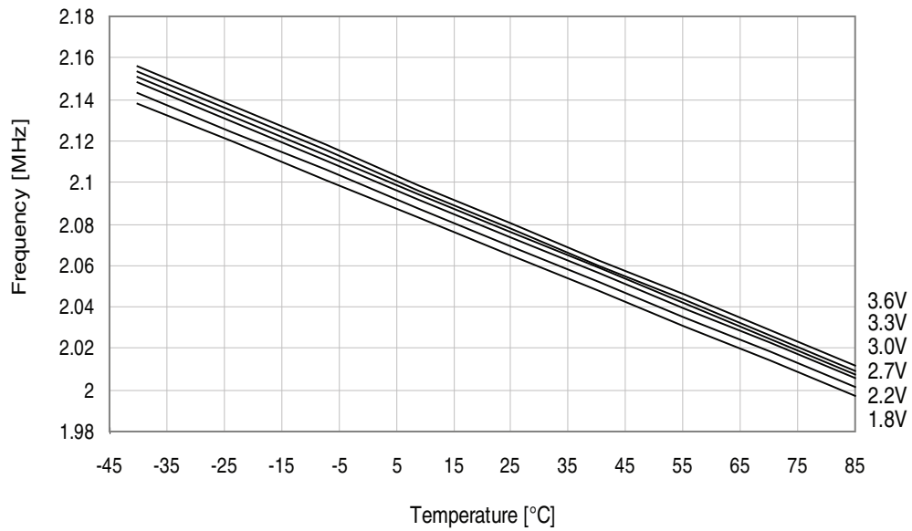
Figure 34-326. 2MHz internal oscillator frequency vs. temperature.
