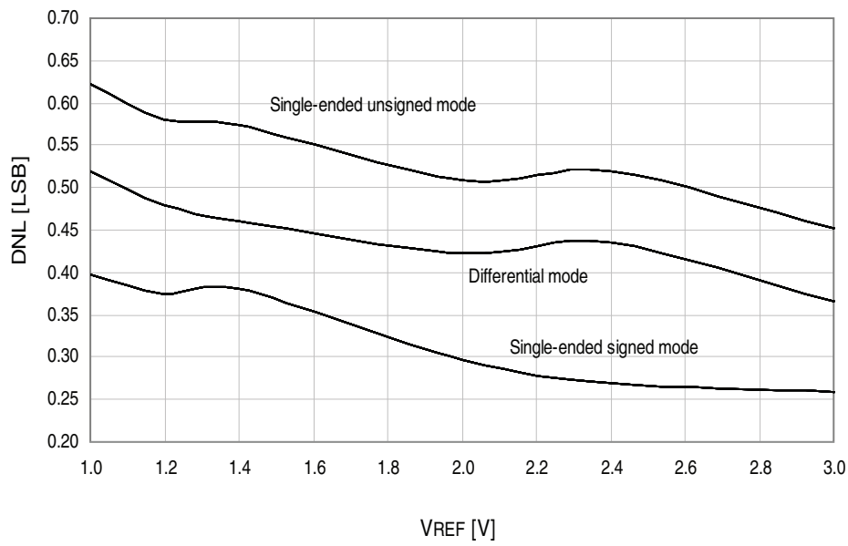
Figure 34-34. DNL error vs. external V_{REF} .
