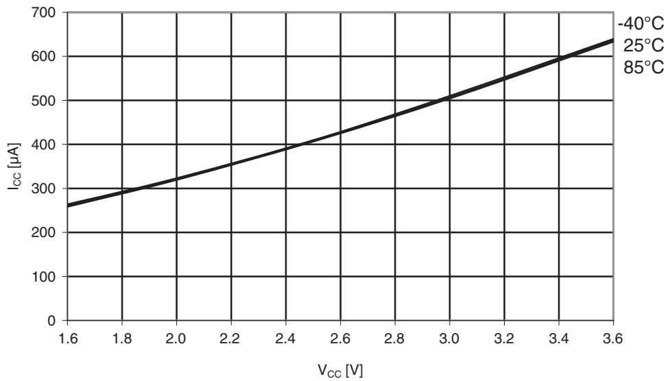
Figure 33-12. Idle supply current vs. V_{CC} . f_{SYS} = 2.0MHz internal RC.
