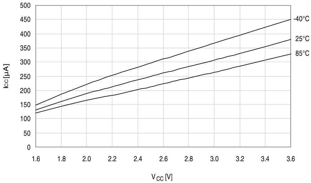
Figure 33-288. Active mode supply current vs. V_{CC} . f_{SYS} = 32.768kHz internal oscillator.
