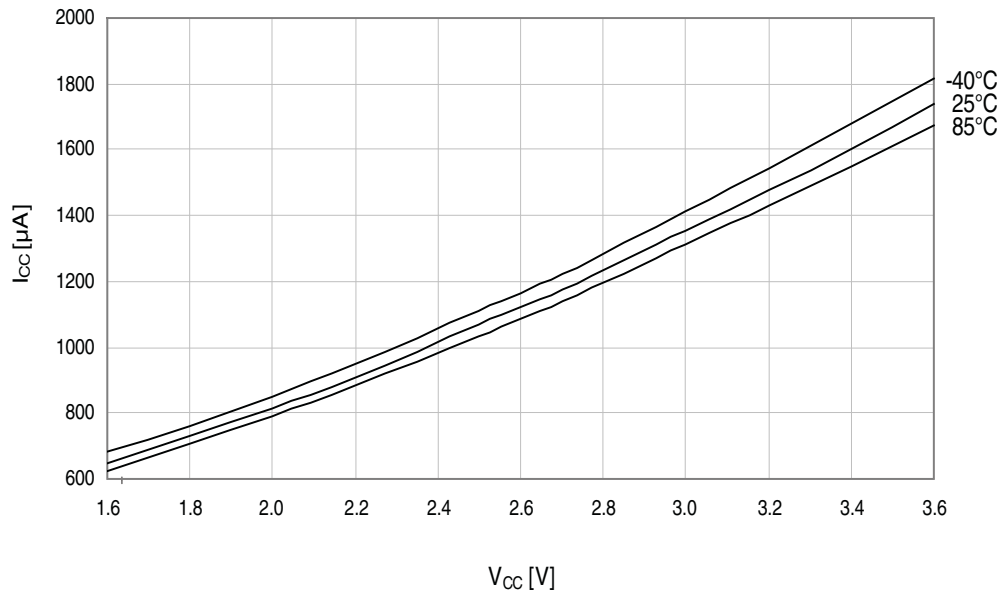
Figure 33-164. Idle mode supply current vs. V_{CC} . f_{SYS} = 32MHz internal oscillator prescaled to 8MHz.
