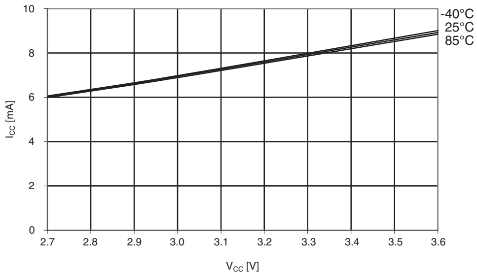
Figure 33-14. Idle supply current vs. V_{CC} . f_{SYS} = 32MHz internal RC.
