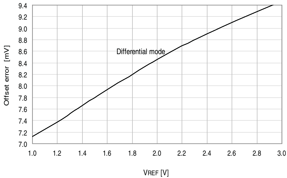
Figure 33-256. Offset error vs. V_{REF} . T = 25^{\circ}\text{C} , V_{CC} = 3.6\text{V} , ADC sample rate = 300kps.
