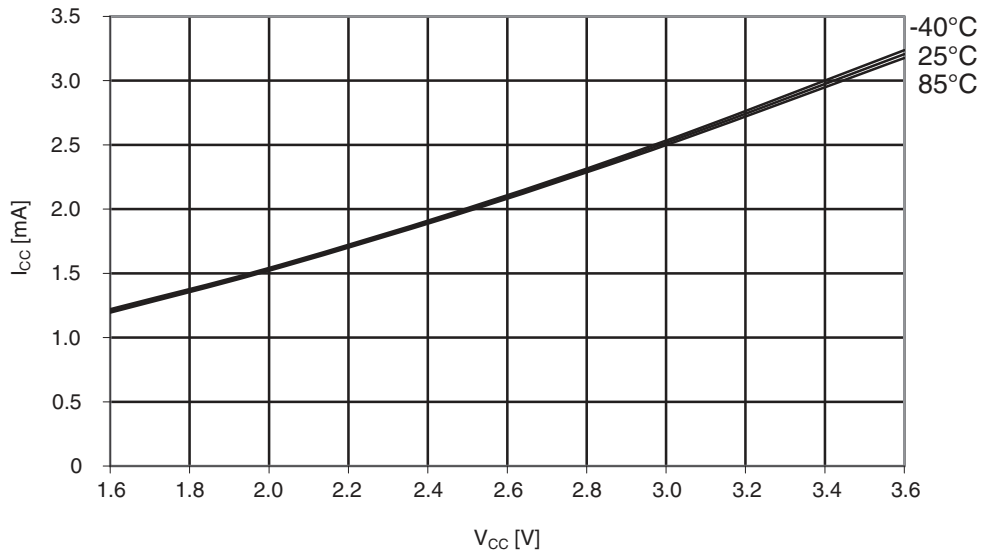
Figure 33-13. Idle supply current vs. V_{CC} . f_{SYS} = 32MHz internal RC prescaled to 8MHz.
