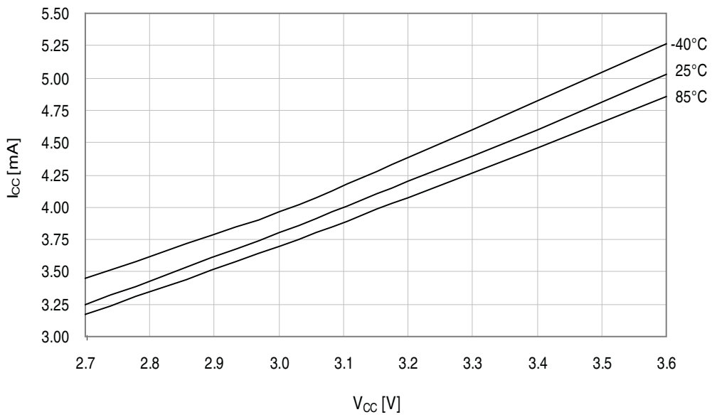
Figure 33-165. Idle mode current vs. V_{CC} . f_{SYS} = 32MHz internal oscillator.
