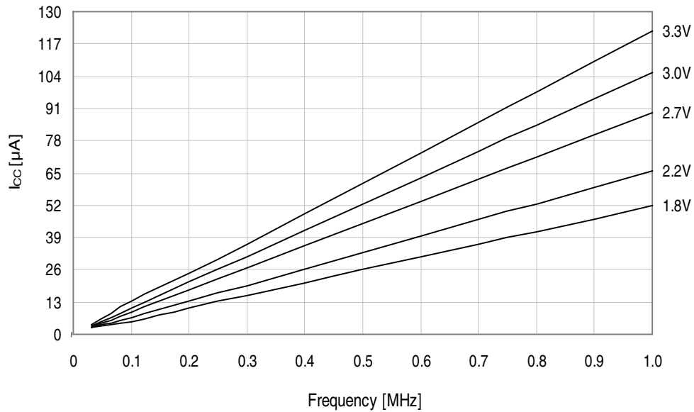
Figure 33-226. Idle mode supply current vs. frequency. f_{SYS} = 0 - 1MHz external clock, T = 25°C .
