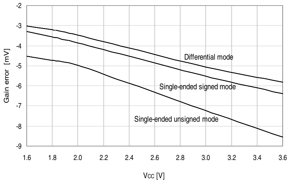
Figure 33-255. Gain error vs. V_{CC} . T = 25^{\circ}\text{C} , V_{REF} = \text{external } 1.0\text{V} , ADC sample rate = 300kps.
