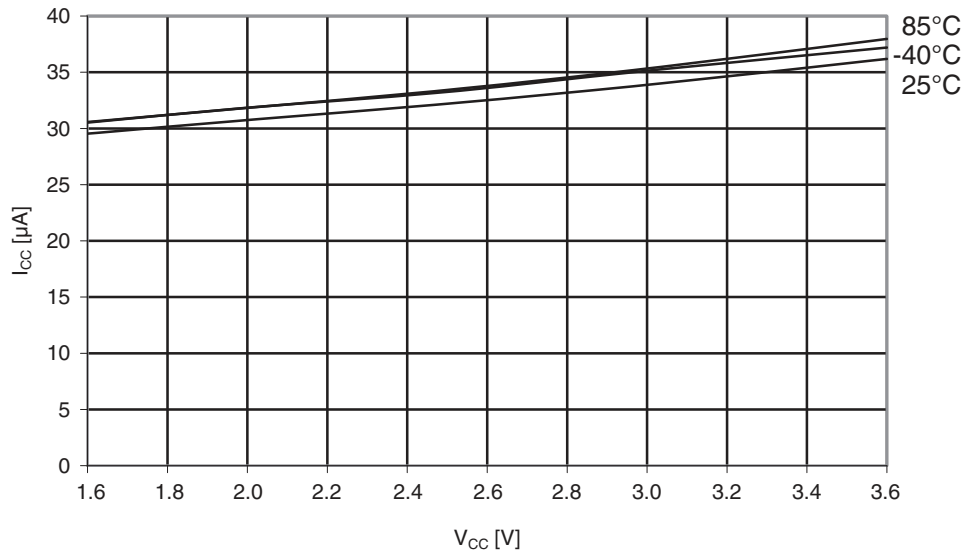
Figure 33-11. Idle supply current vs. V_{CC} . f_{SYS} = 32.768kHz internal RC.
