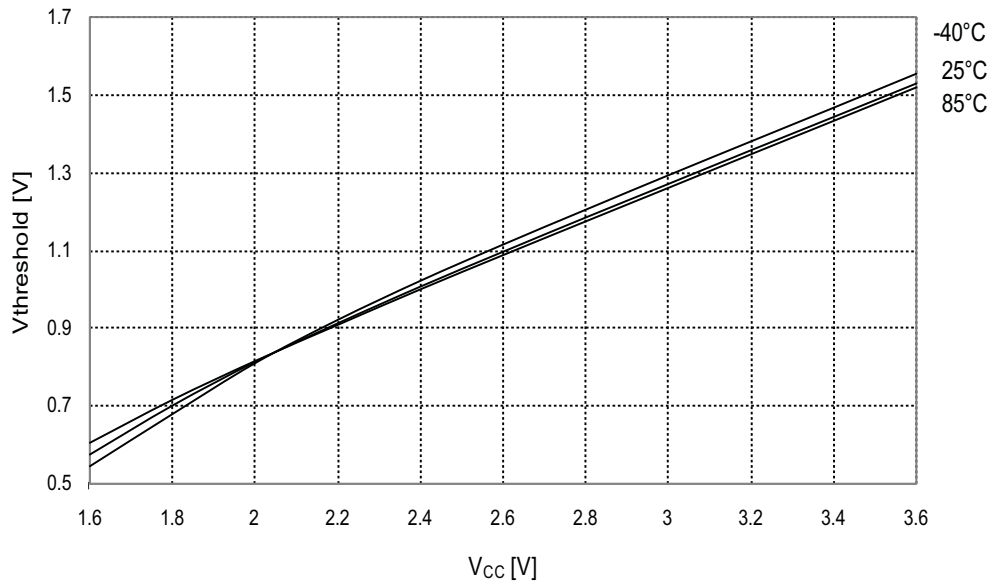
Figure 33-112. I/O pin input threshold voltage vs. V_{CC} .
