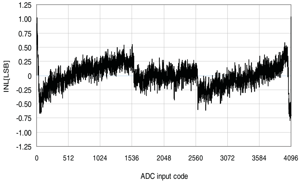
Figure 33-317. INL error vs. input code.
