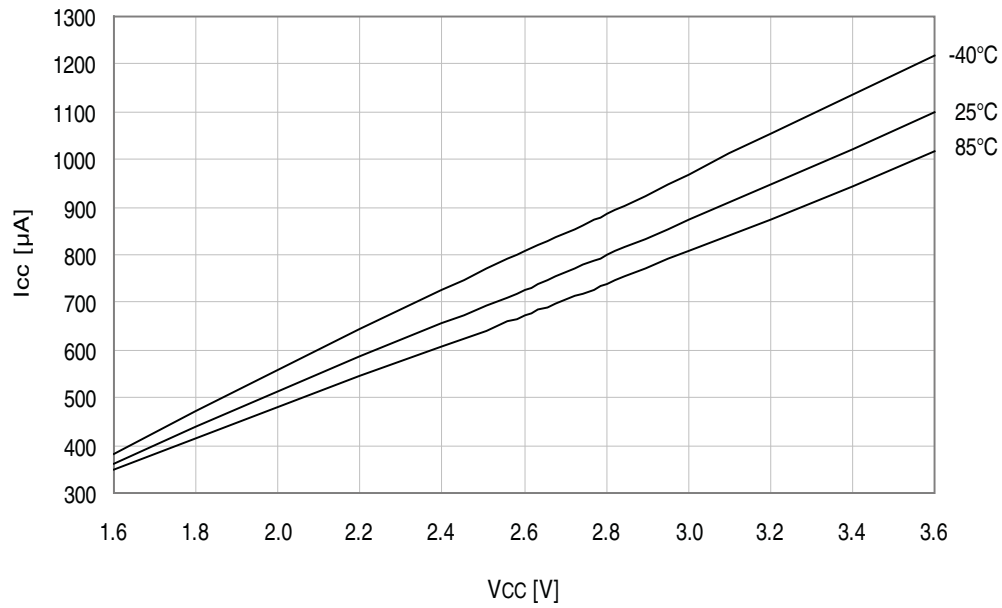
Figure 33-289. Active mode supply current vs. V_{CC} . f_{SYS} = 1MHz external clock.
