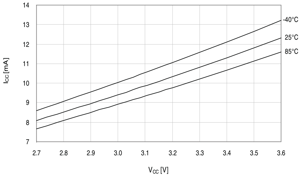
Figure 33-225. Active mode supply current vs. V_{CC} . f_{SYS} = 32MHz internal oscillator.
