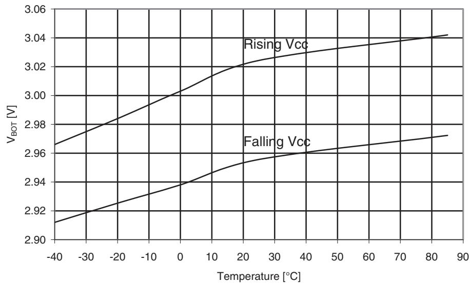
Figure 33-33. BOD thresholds vs. temperature.
