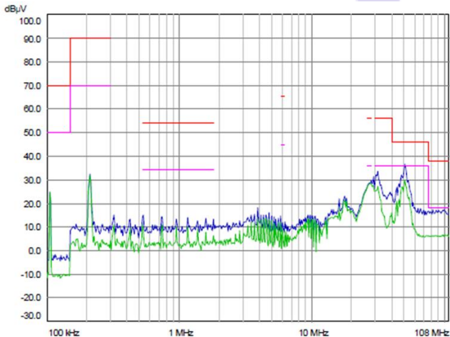
CF0505XT-1WR2 CE(Positive line)
