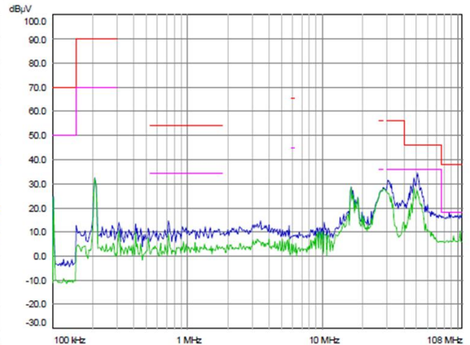
CF0505XT-1WR2 CE(Negative line)
