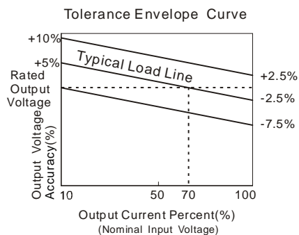
CF0505XT-1WR2 CE(Positive line)
