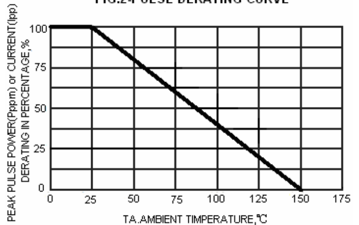
FIG.2-PULSE DERATING CURVE
