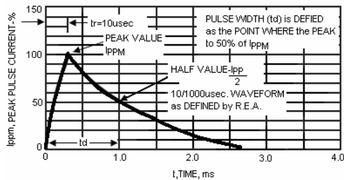
FIG.3-PULSE WAVEFORM
