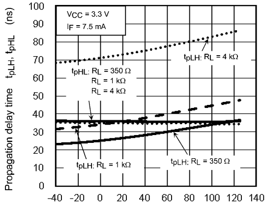
Fig. 12.2.13 t_{pLH}, t_{pHL} - T_a
