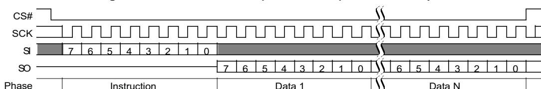
Figure 114. Password Read (PASSRD E7h) Command Sequence
