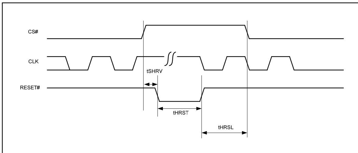
Figure 33. Reset Timing
