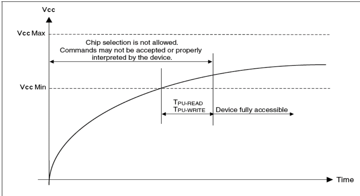
Figure 28. Power-up Timing
