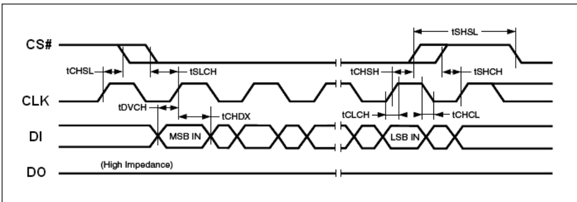
Figure 31. Input Timing
