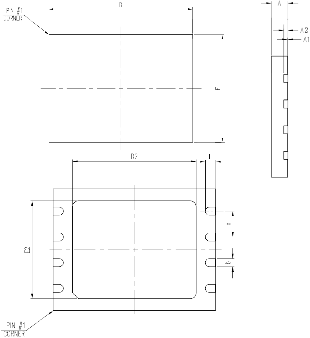
Figure 35. VDFN8 ( 5x6mm )
