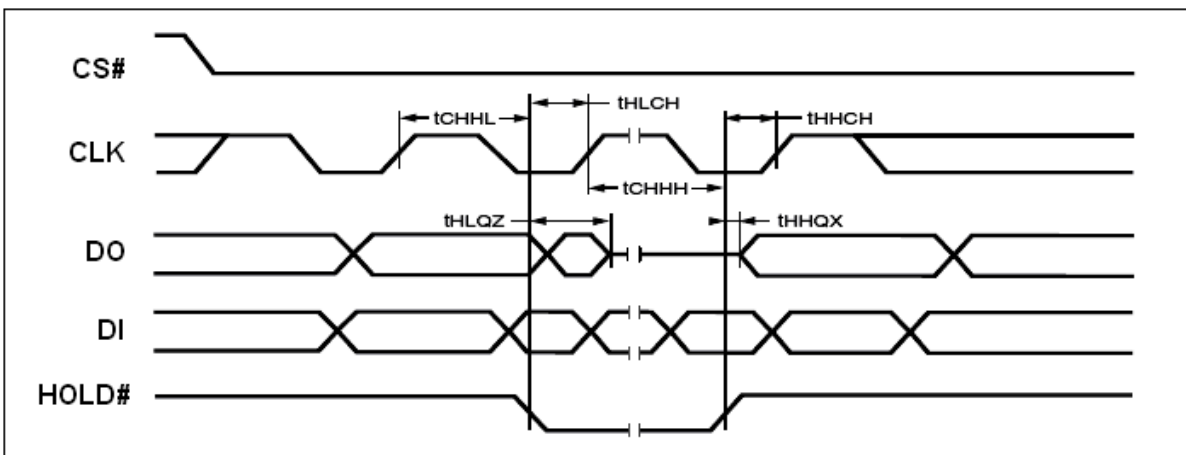
Figure 32. Hold Timing
