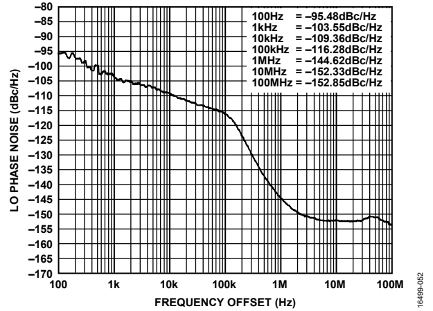
Figure 127. LO Phase Noise vs. Frequency Offset, LO = 525 MHz, PLL Loop Bandwidth = 50 kHz
