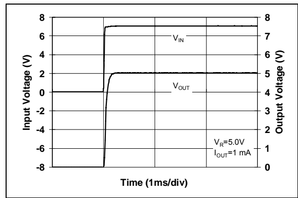
FIGURE 2-36: Startup Response.
