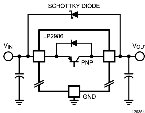
FIGURE 2. Adding External Schottky Diode Protection
