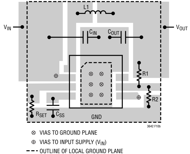
Figure 10. Layout Example
