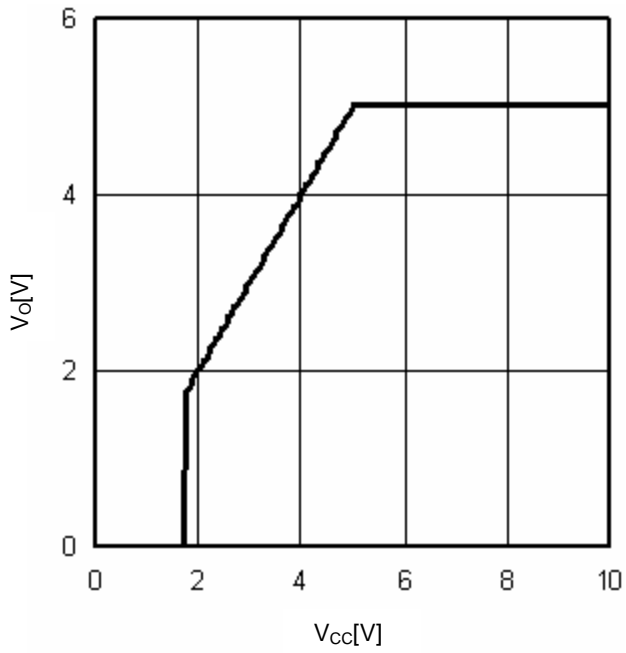
Fig.14 V_{CC}-V_O ( I_o=0mA )
