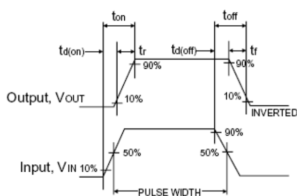
Switchin Waveforms
