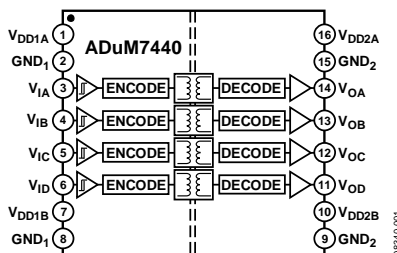
Figure 1. ADuM7440
