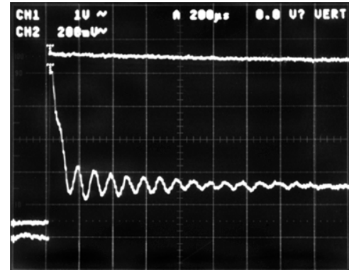
Figure 11. Typical Self-Test Response at V_{DD} = 5\text{ V}
