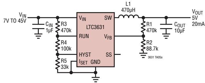
Small Size, Limited Peak Current, 20mA Regulator
