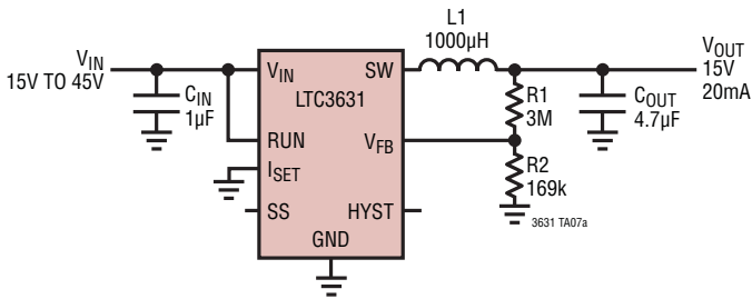
High Efficiency 15V, 20mA Regulator
