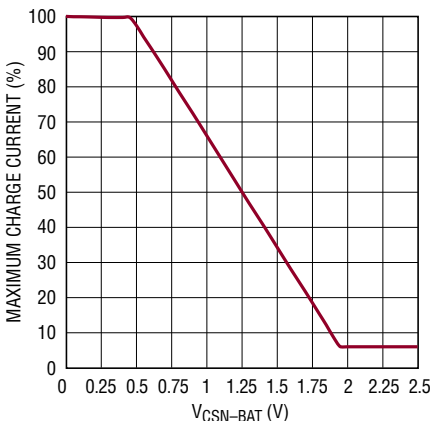
Instant-On: Maximum Charge Current (Percent of I CSMAX ) vs V CSN-BAT
