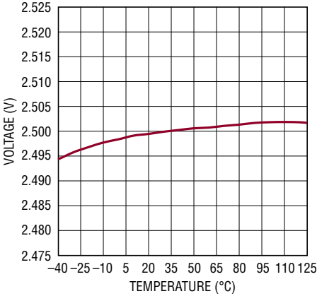
V FLOAT(CC/CV) OR, V ABSORB(Lead-Acid) Reference vs Temperature
