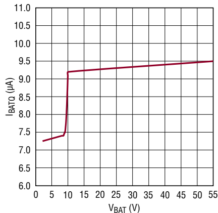
I BATQ (I BAT + I CSN + I CSP ) vs V BAT PowerPath Switcher Disabled
