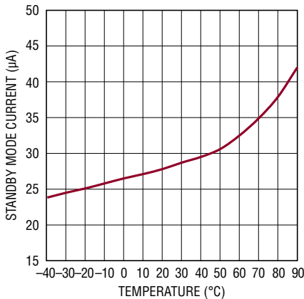
Shutdown Current vs Temperature (I PVIN + I SENSVIN + I SENSTOP )
