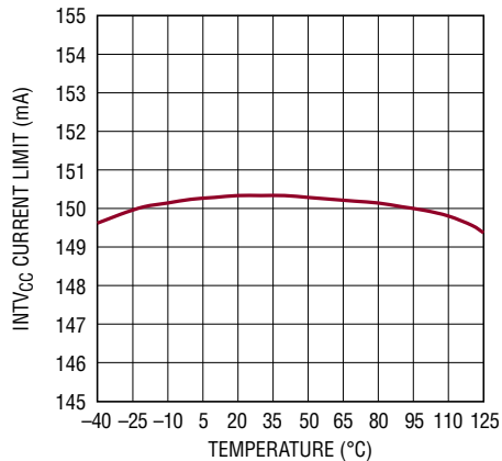
INTV CC Short-Circuit Current Limit vs Temperature
