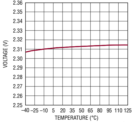
V FLOAT(Lead-Acid) Reference vs Temperature
