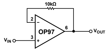
Figure 33. Unity-Gain Follower
