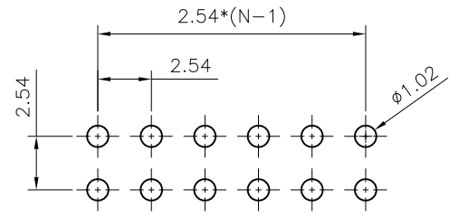
RECOMMEND PCB LAYOUT (TOLERANCE ±0.05)
