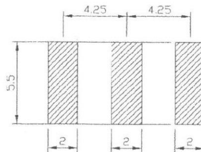
REFERENCE P.C.H LAYOUT
