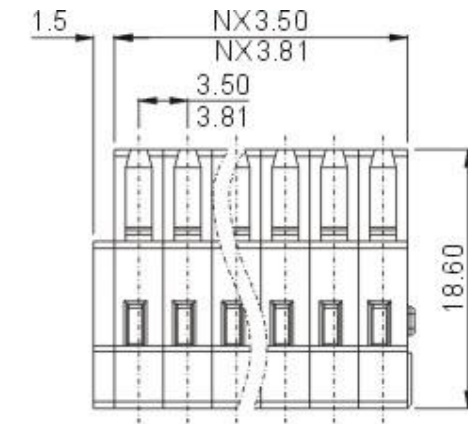
8EDGK-3.5 8EDGK-3.81
